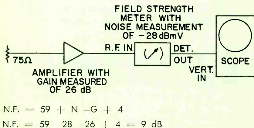
Fig. 2 Example of noise figure calculation of an amplifier. Observe scope trace such that only noise is seen, no video or FM pickup.
