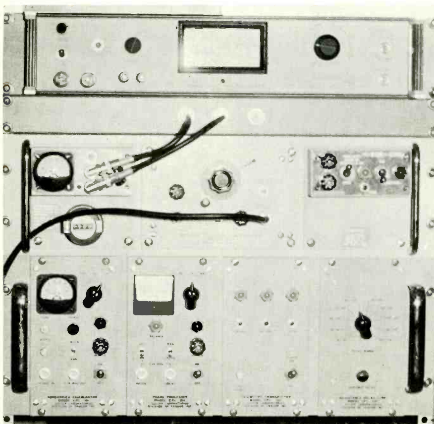
Fig. 8 Second unit from bottom is the NYN time standard. Across the bottom from left to right are the subcarrier regenerator, phase processor, telemetry transmitter, and the adjustable delay line.
